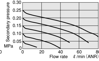
MRN1□1-J4, J1/8
