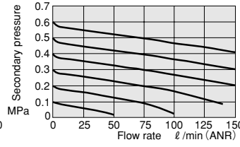
MRN1□0-J6, J1/4
